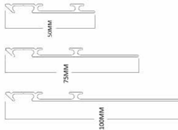
Skirting Profile 50, 75 & 100 mm
